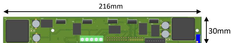
Top view
